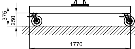
Lasthaken E 012 - P
